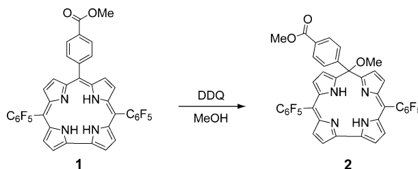
Scheme 1. Conversion of corrole 1 to isocorrole 2 .
